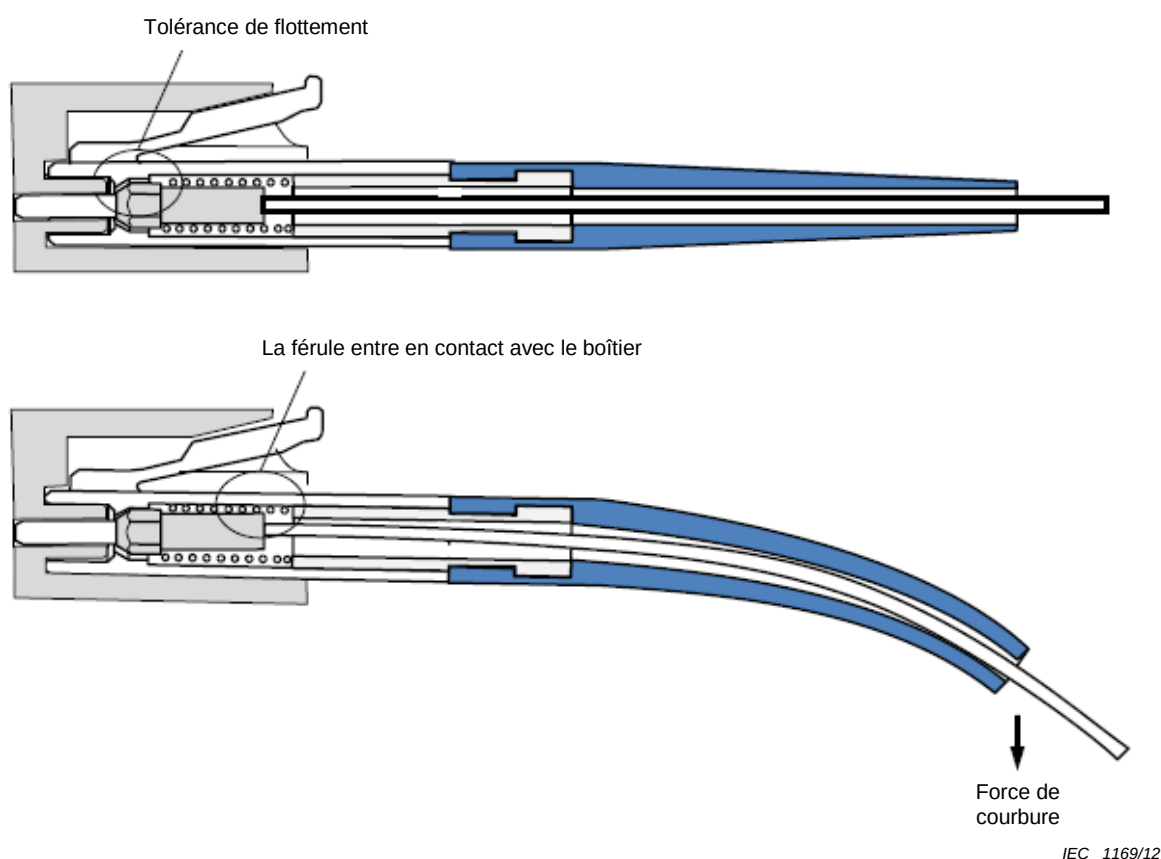
Figure D.1 – Tolérance de flottement
