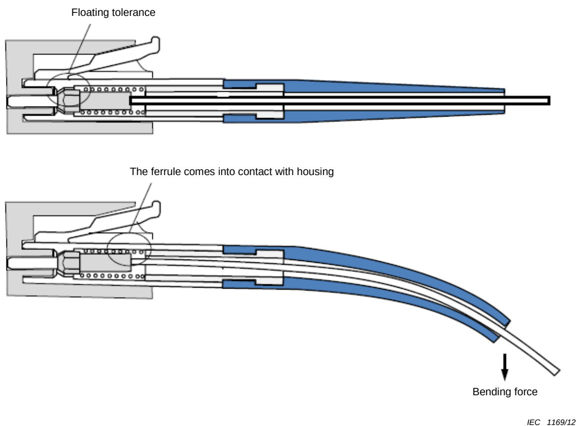
Figure D.1 – Floating tolerance
