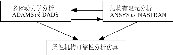
图 4 机构可靠性综合分析仿真 Fig. 4 Integration of multibody dynamics, strength and mechanism reliability simulation
